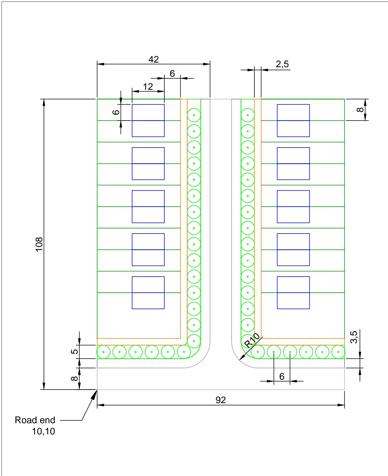
Autocad Exercise Street Layout
